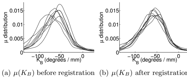
Fig. 3. Effect of registration and shape normalization on K_B . (a) Computing the GHM parameters on the original hearts produces unaligned K_B distributions. (b) The group-wise registration process yields aligned K_B distributions.
