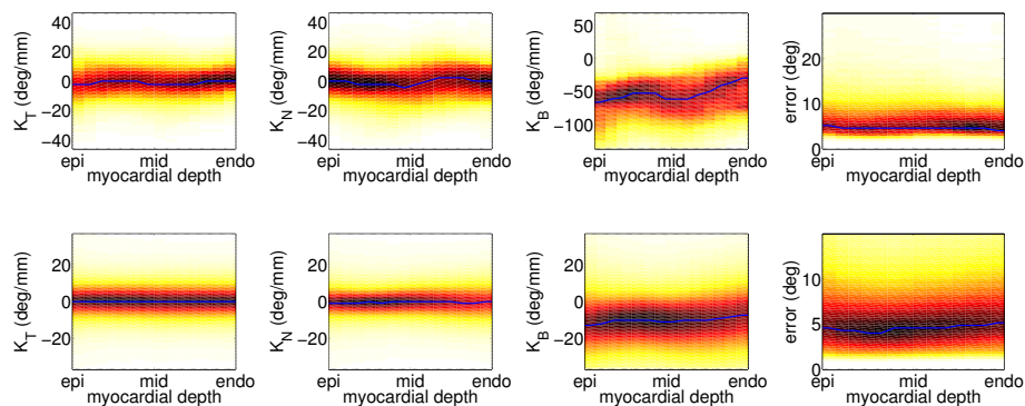
Fig. 5. Transmural distribution ( y axis) of the GHM parameters K_T , K_N , K_B and fitting error as a function of transmural depth ( x axis) from epicardium to endocardium for the rat (top) and canine (bottom). The coloring shows the probability distribution of a GHM parameter at a particular transmural depth, and blue lines join the distribution modes along the transmural depth.
